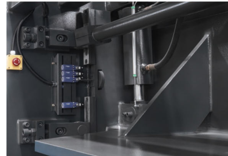
Adjust Blade Clearance With Upper Fulcrum
